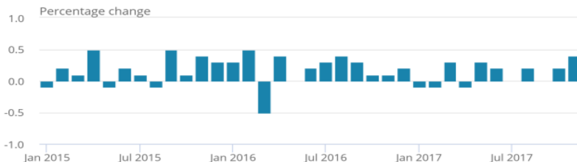
Index of Services headline growth rates from January 2015 to November 2017
